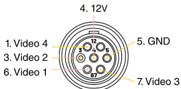
Pin Diagram Cable Female
