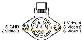
Pin Diagram Cable Male
